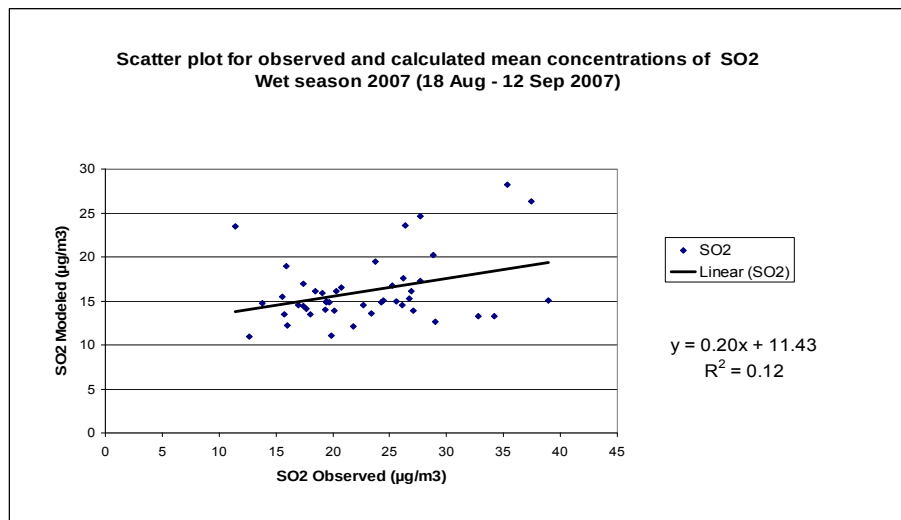
Figure 6.21. Scatter plot for observed and calculated mean concentrations of SO 2 – Wet season 2007 (µg/m 3 ).
