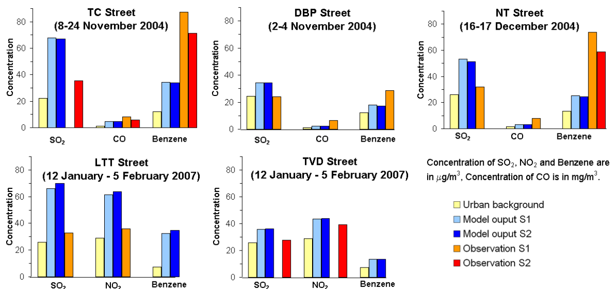
Figure 5.49. Modelled and observed mean concentrations for the five selected streets. Urban background concentrations are also provided for reference.
