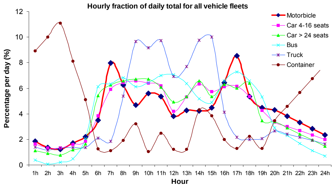
Figure 3. Average diurnal variation of the six vehicle categories plotted as hourly fraction (in %) of the daily total of each vehicle category. Based on data from 43 locations. (Source: JICA & TEDI, 2006)
