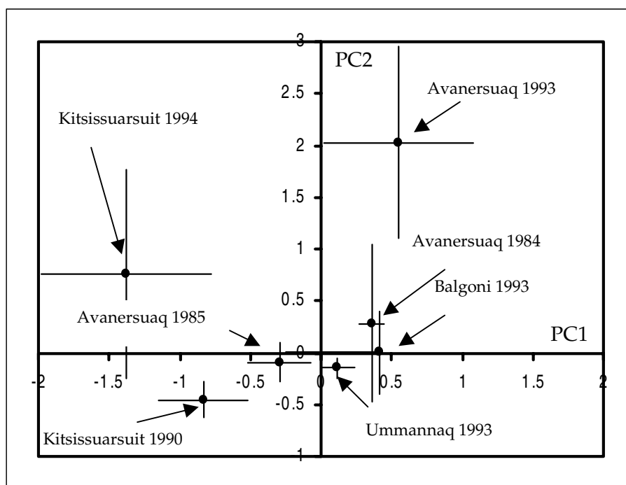
Figure 3.3.3. PCA analysis on PCB congeners in narwhals. Plot of mean and standard errors of PC1 versus PC2.
