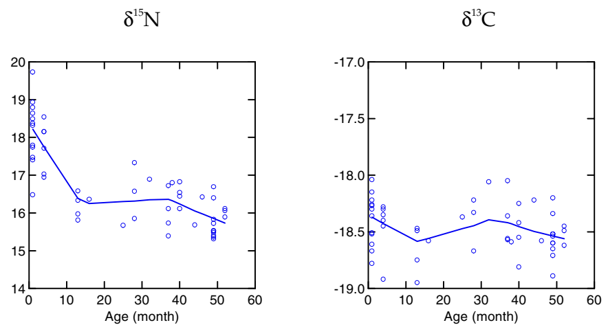
Figure 3.4.1. Relationship between stable isotopes and age. Lines represent LOW-ESS smoother.
