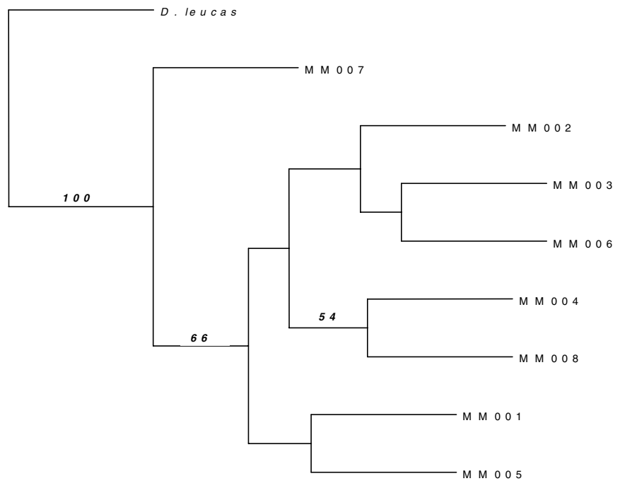
Figure 3.5.1. The genealogy estimated from the eight narwhal haplotypes and rooted with the homologous beluga sequence. Note: Numbers indicate bootstrap values in percent (only values over 50 included)
